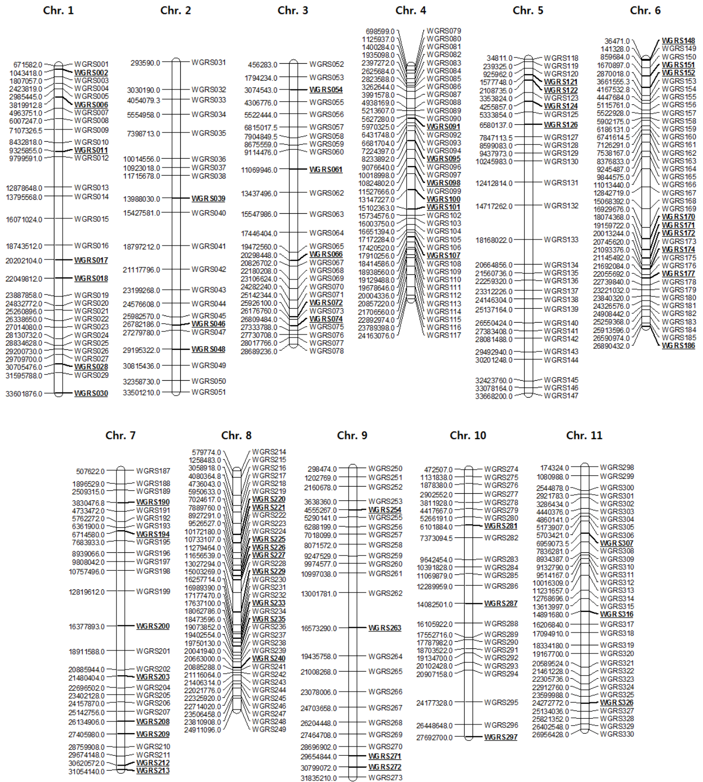
Supplementary Fig. 1. Position of 330 HRM primer sets on physical map of watermelon. Especially, underlined and bold marker name means polymorphic HRM markers between ‘920533’ and ‘PI 189225’.
